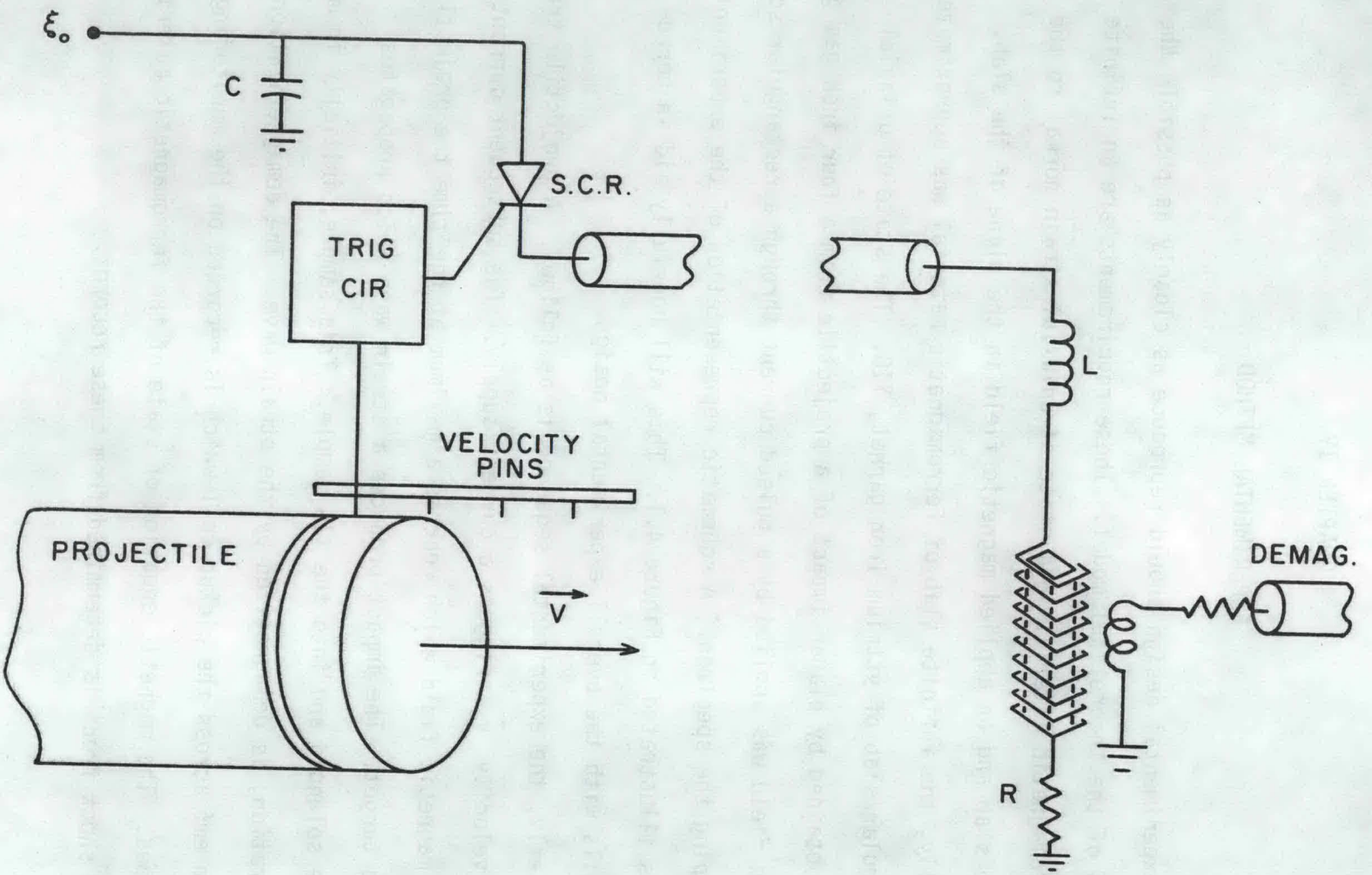
Fig. 4.1.--Schematic representation of experimental method.
